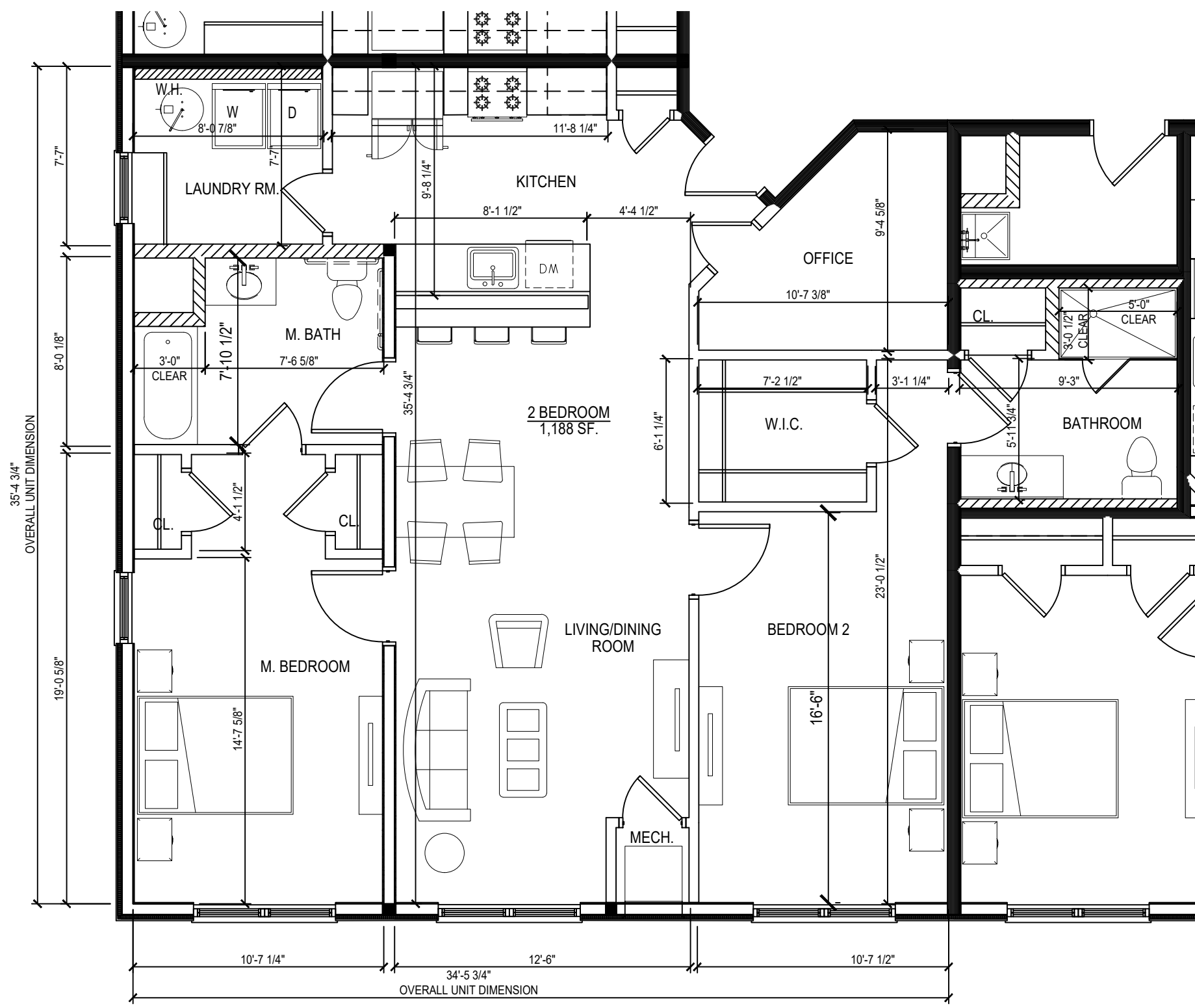
1 UNIT 113 - 2 BDRM - 1,188 S.F. SCALE: 3/16"=1'-0"
